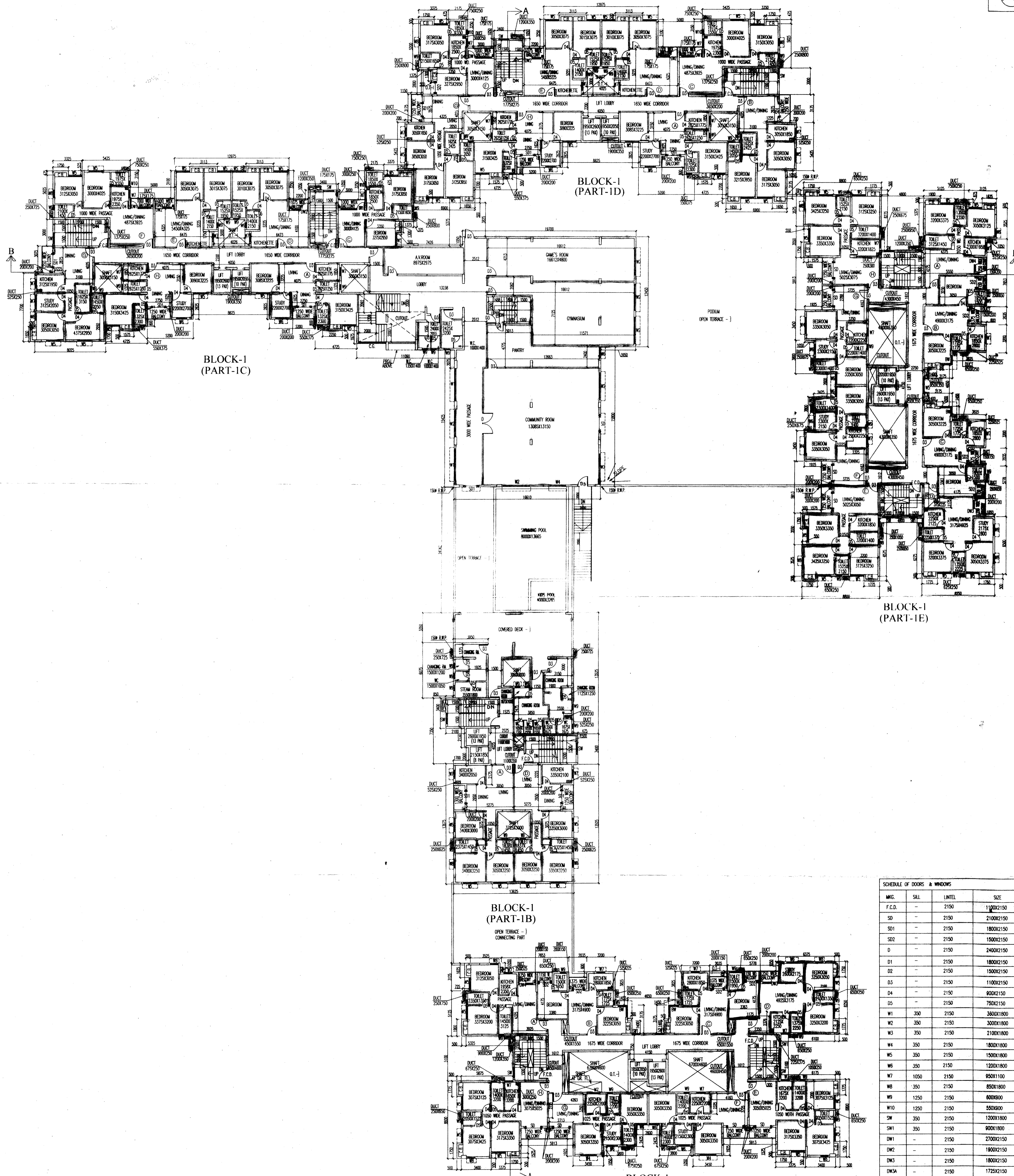
OVERALL FIRST FLOOR PLAN SCALE - 1 : 200
